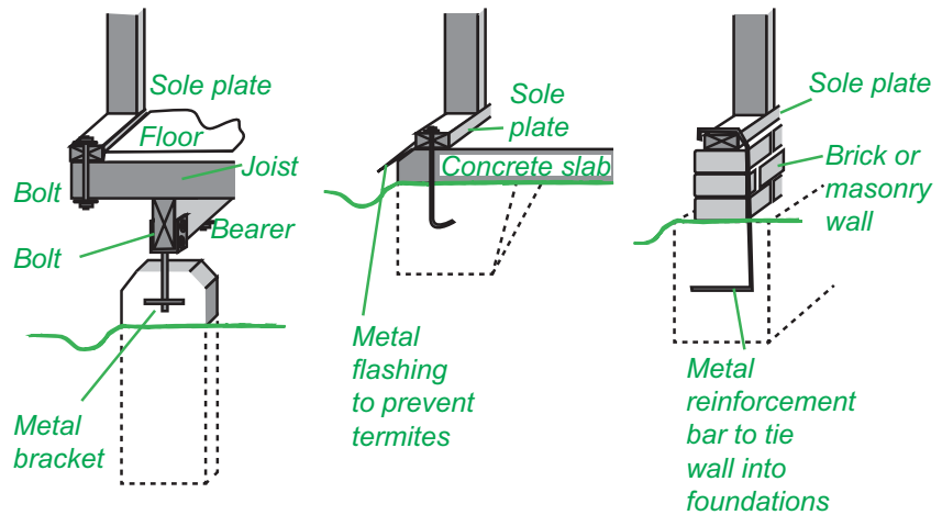
Pad foundation raised floor
